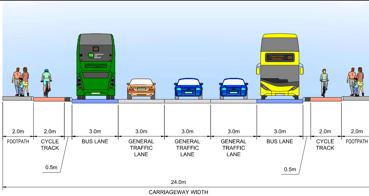
TYPICAL SECTION I-I DUBLIN ROAD LOCATED ON GA SHEET 09 DRAWING REF: BCGDR-BTL-GEO_GA-XX-DR-CR-00009
