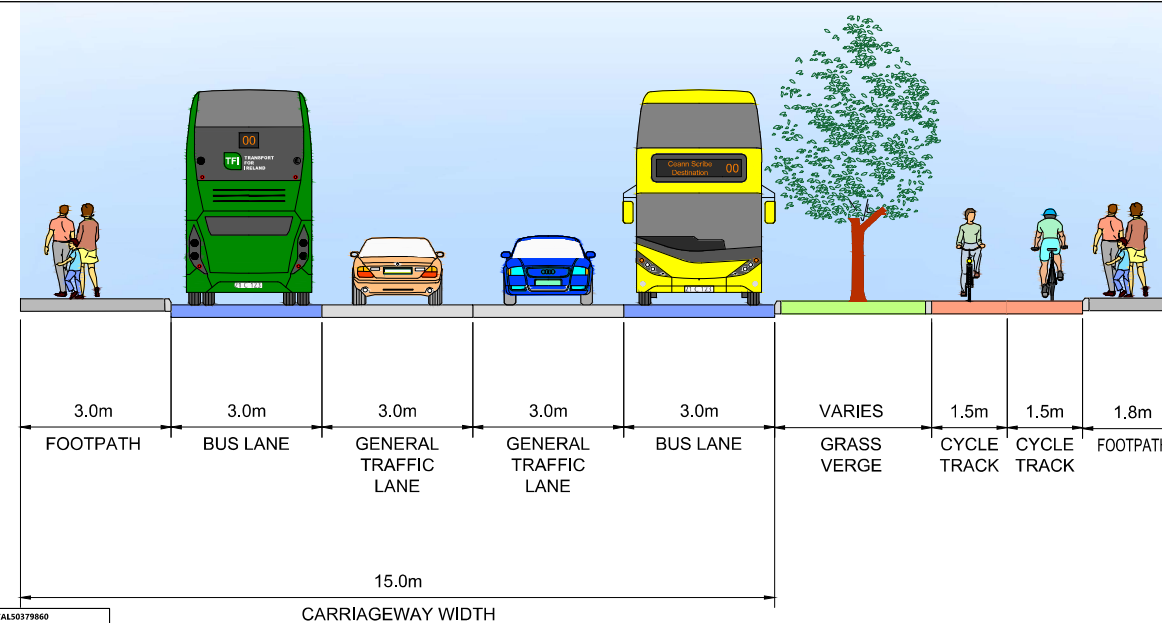
TYPICAL SECTION J-J DUBLIN ROAD LOCATED ON GA SHEET 10 DRAWING REF: BCGDR-BTL-GEO_GA-XX-DR-CR-00010
